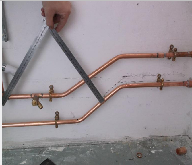
Task 2 Photo ref 13. Offset bends not parallel. 100mm centres in mid-point range from 85mm to 110mm across the length of offsets. Munson clips not aligned with each other.
